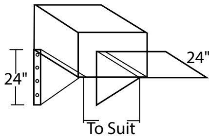
WALL MOUNTED CHARGER SUPPORT
